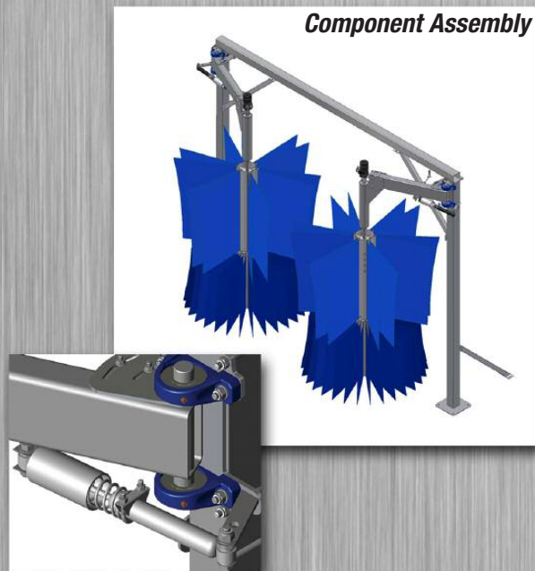
Component Assembly
